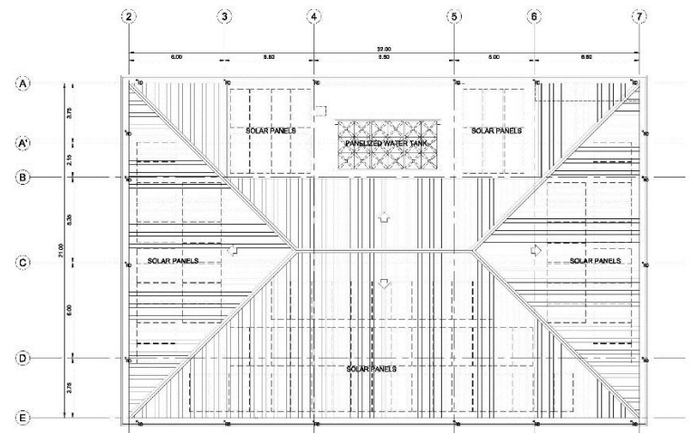
ROOF PLAN
