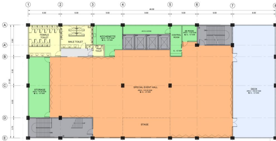
SEVENTH FLOOR
